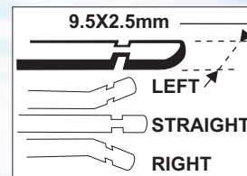
WIPER ARM ROD WIDTH DIMENSION
